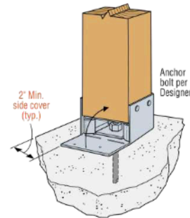
Typical ABWZ Installation
