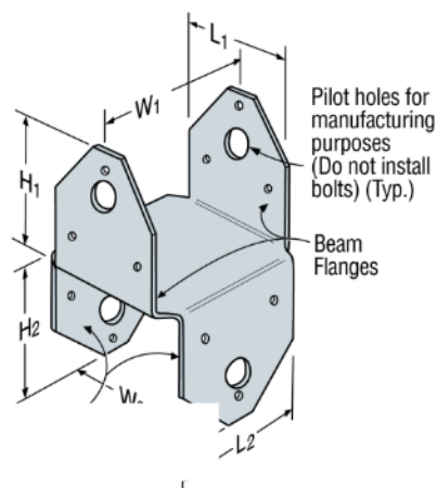
Typical BCS Post Cap Installation
