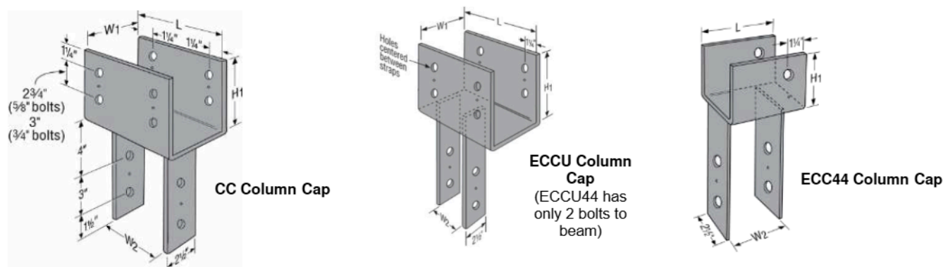
FIGURE 1—CC AND ECC COLUMN CAPS
