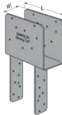
ECCQ46SDS2.5 Column Cap for End Conditions
