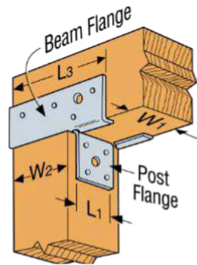
Typical EPC End Post Cap Installation
