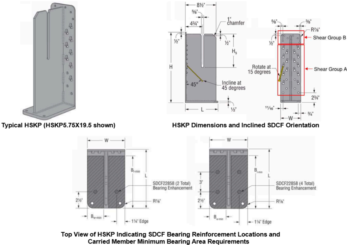
FIGURE 20—HEAVY SEATED KNIFE PLATE HANGER
