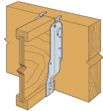
FIGURE 15C—TYPICAL IUS HANGER INSTALLATION (Supported Wood I-joist without Web Stiffeners)
