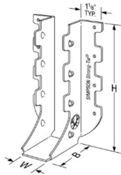
FIGURE 7—MUS HANGER (See Table 7 )
