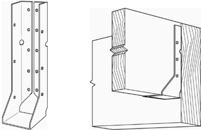
FIGURE 2—LUCZ SERIES HANGER AND INSTALLATION DETAIL
