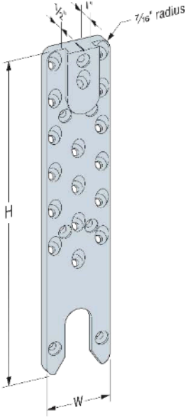
SCBH Series Hanger
