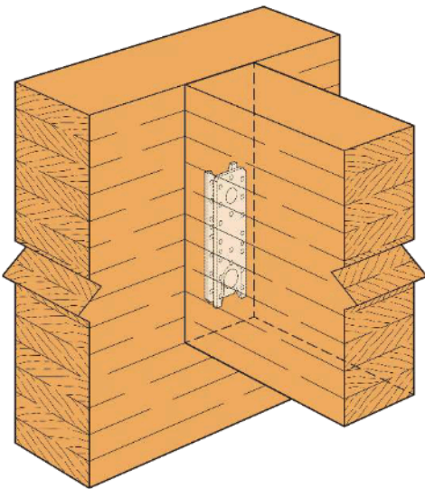
Typical CBH Beam-Beam Installation Beam-Column Installation Similar
