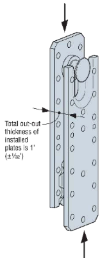
Typical CBH Assembly
