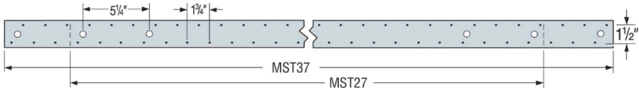
FIGURE 27—MST STRAPS
