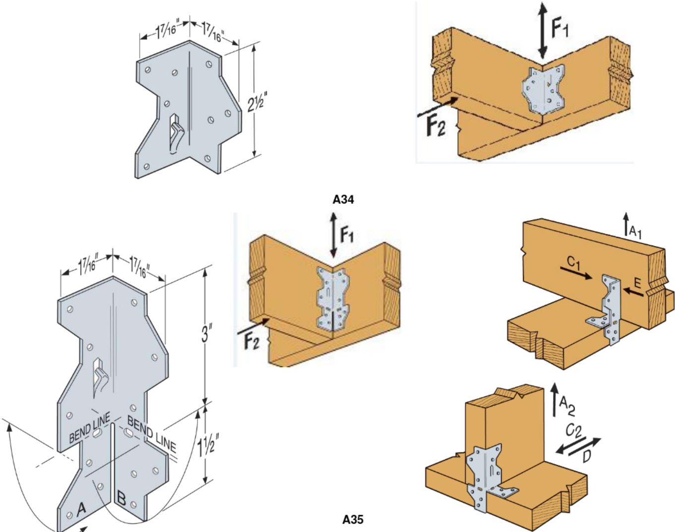
FIGURE 5—A ANGLES
