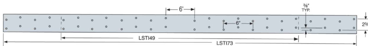
FIGURE 29—LSTI STRAPS
