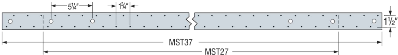
FIGURE 27—MST STRAPS
