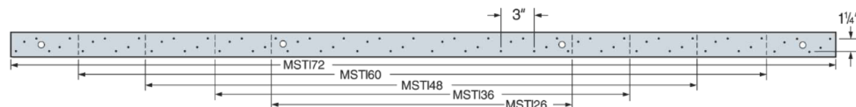
FIGURE 30—MSTI STRAPS
