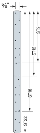
FIGURE 24—ST STRAPS
