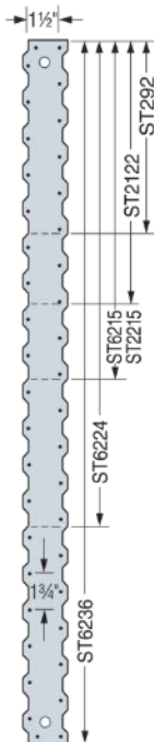
FIGURE 25—ST STRAPS
