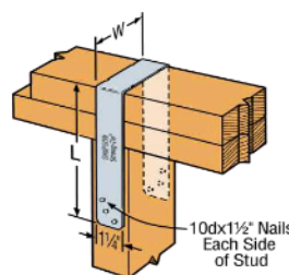
Typical SP4 Installation: Double Top Plate
