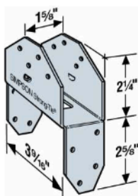
HS24 Dimensions U.S. Patents 5,603,580
