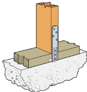
SSP Installation: Single Stud to Sill Plate
