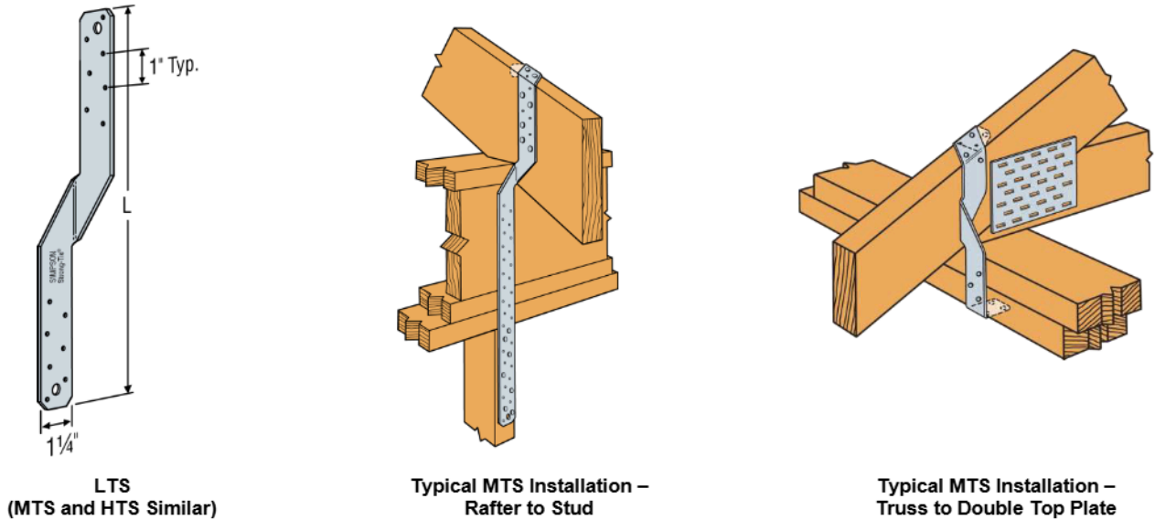
FIGURE 3—TWIST STRAPS
