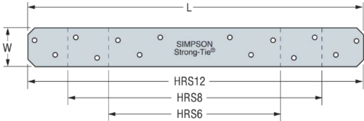
FIGURE 33—HRS STRAP
