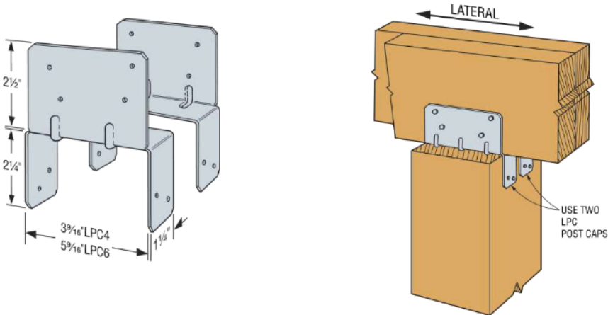
FIGURE 14—LPC SERIES
