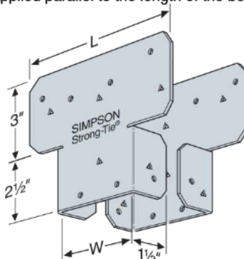
FIGURE 10—AC SERIES
