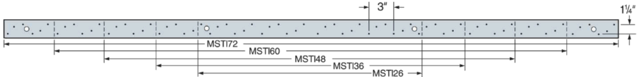
FIGURE 30—MSTI STRAPS
