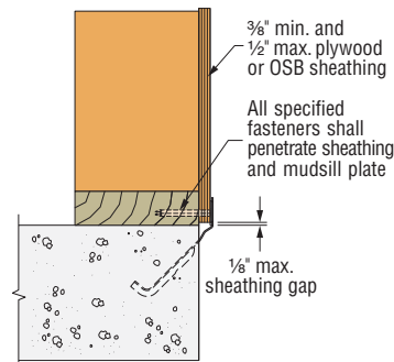
Typical MASOZ/MASOPZ Final Installation with Overhanging Sheathing
